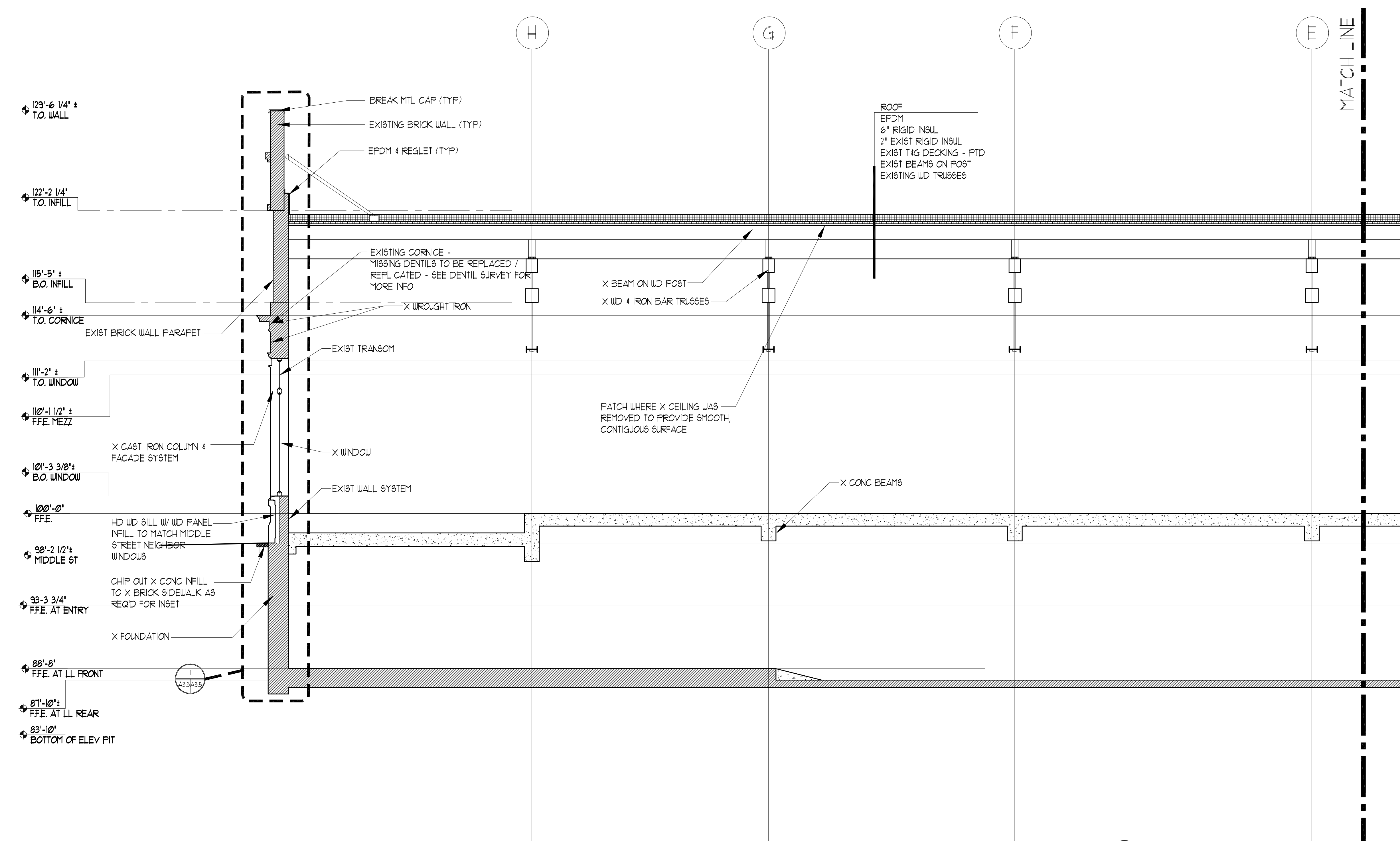
BUILDING SECTION SCALE: 1/4" = 1'-0"
